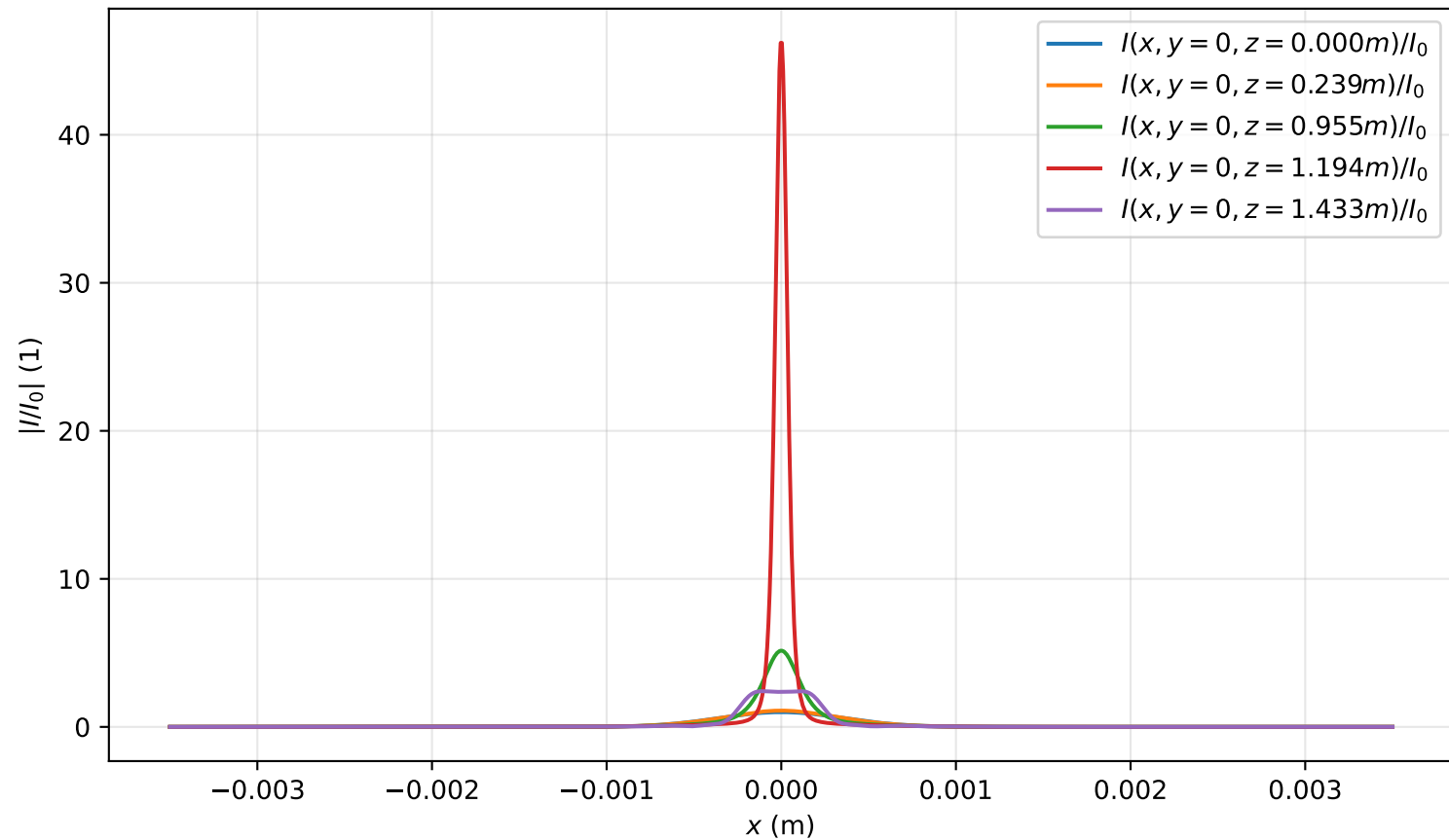
Intensity profile I(x, y = 0, z)/I_0 , Pin=1.9Pcr, artificial time
